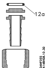
Fig. 2, Fittings for hose connection-outlet incl. O-ring
