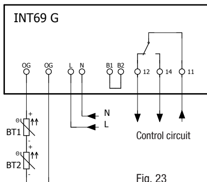
Fig. 23 Terminal box
