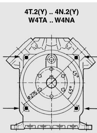
Fig. 5 Fixing positions for coupling housing
